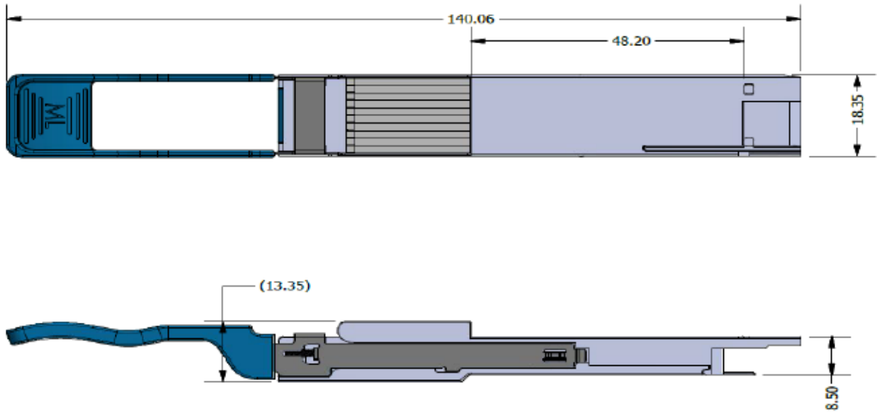
Figure 9: Mechanical Dimensions
